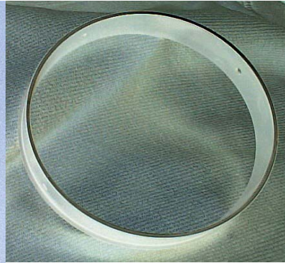
Main bearing liner for the Pratt and Whitney R1340 Wasp series engines used to power T-6 Texans racing at Reno.
