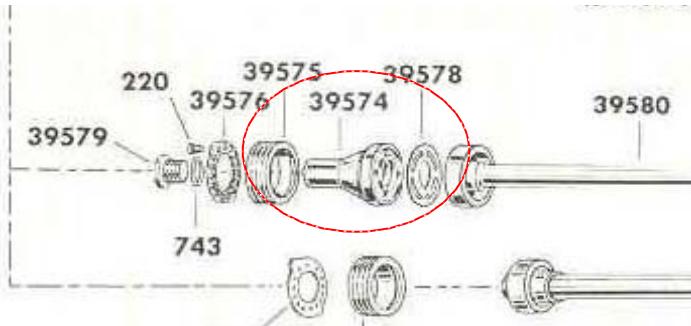
Left: FAA-PMA ASC39574 - Pratt & Whitney Aircraft R985 Wasp Jr. - Crankshaft Plug Below: FAA-PMA ASC39785 Pin Assembly for Pratt & Whitney Aircraft R985 Wasp Jr Articulated Rod.
