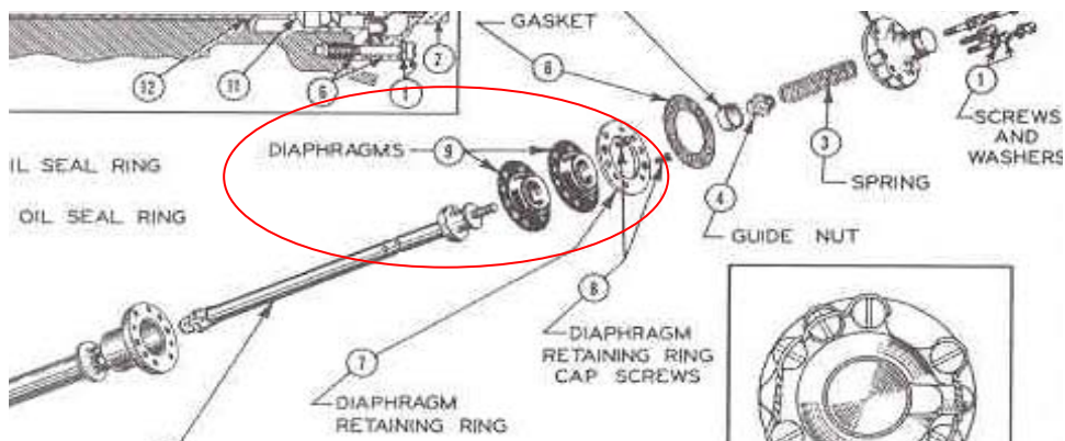
FAA-PMA ASC235257 Diaphragm for Fuel Feed Valve installed on Pratt & Whitney Aircraft R2800 Double Wasp Engines
