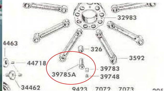
Left: FAA-PMA ASC39574 - Pratt & Whitney Aircraft R985 Wasp Jr. - Crankshaft Plug Below: FAA-PMA ASC39785 Pin Assembly for Pratt & Whitney Aircraft R985 Wasp Jr Articulated Rod.
